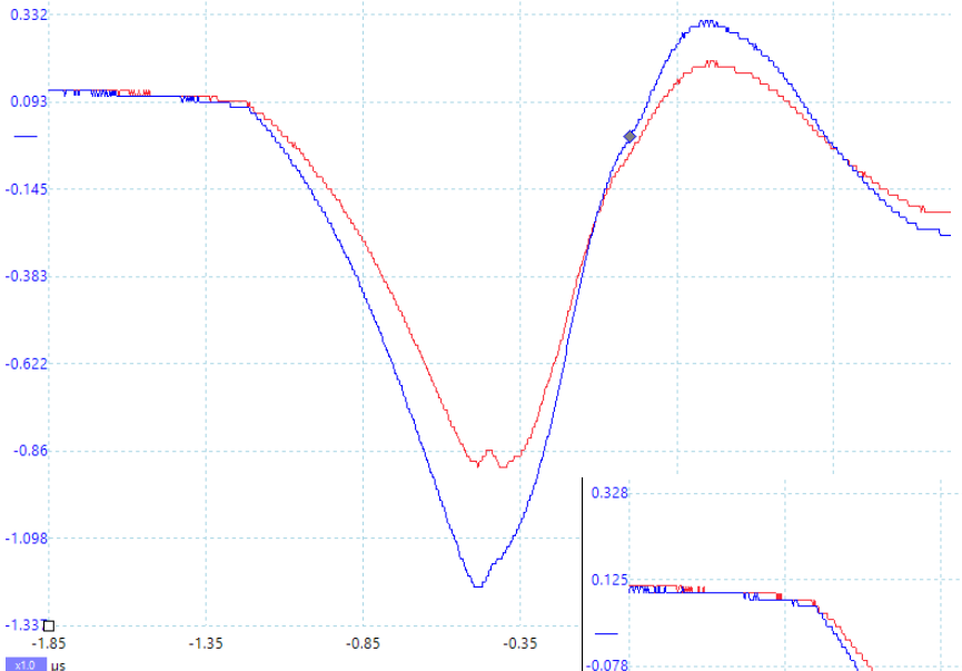
Probe 1 ChA, Transistor1 base Probe 2 ChB, Transistor4 base
