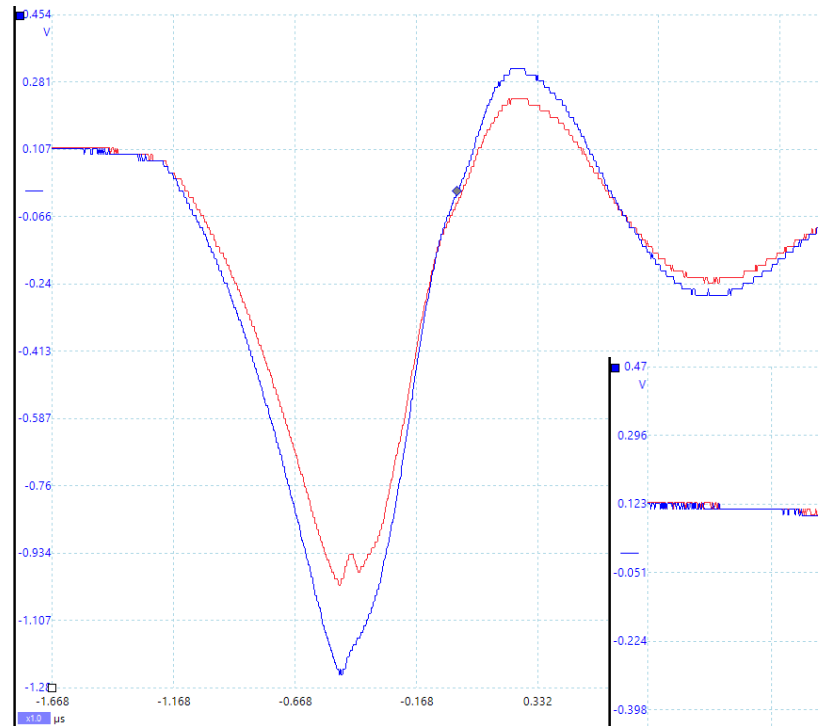
Probe 1 ChA, Transistor1 base Probe 2 ChB, Transistor2 base
