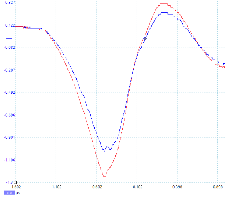
Probe 1 ChB, Transistor1 base Probe 2 ChA, Transistor4 base
