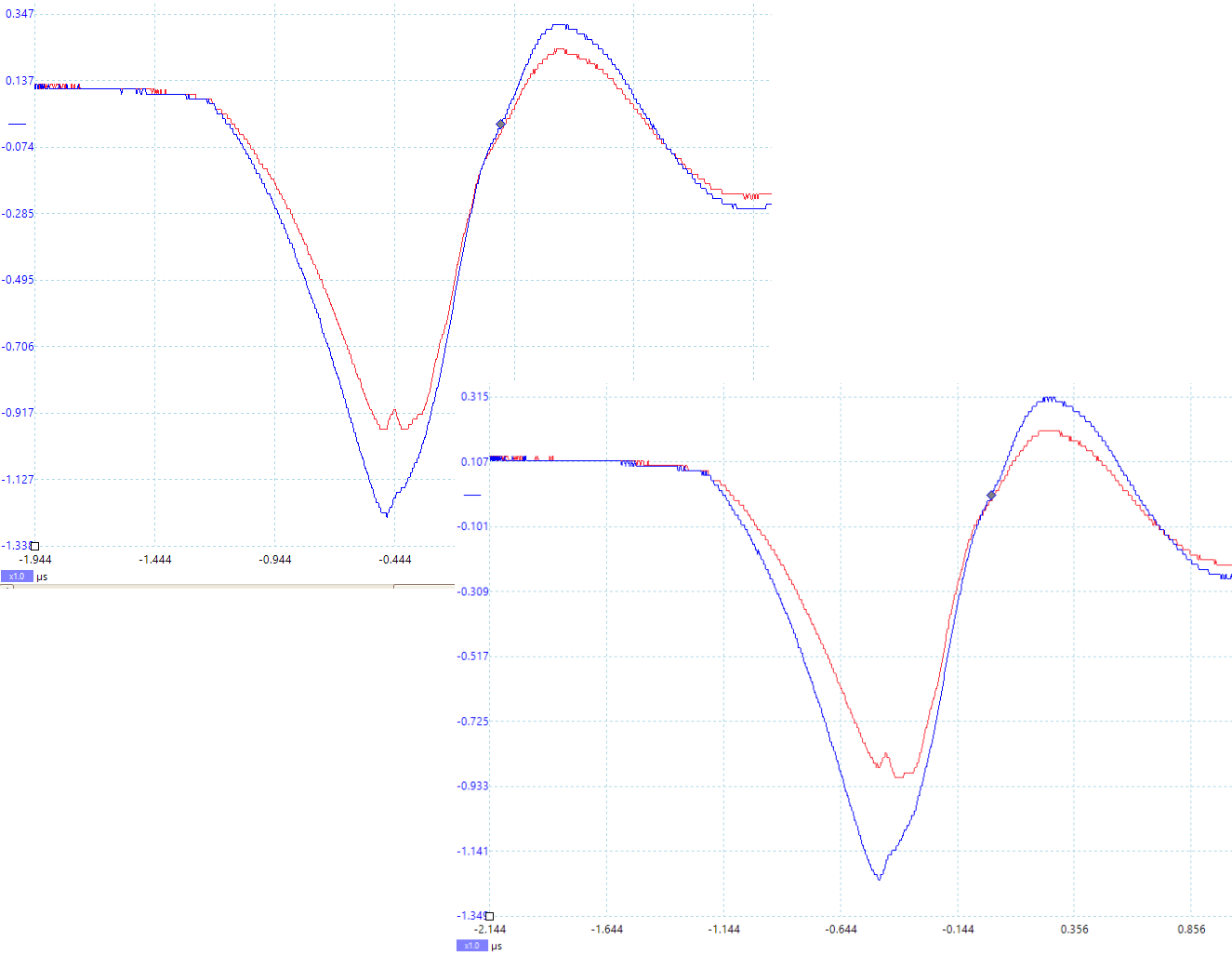
Probe 1 ChA, Transistor1 base Probe 2 ChB, Transistor5 base
