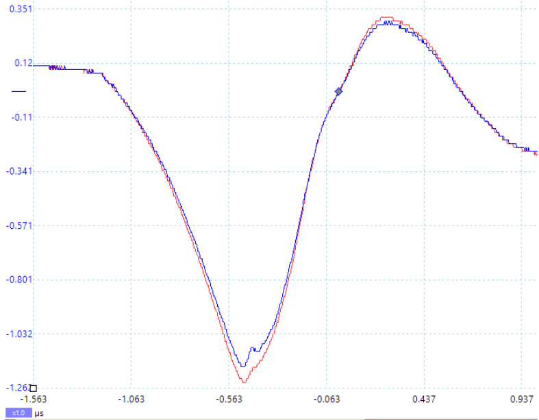
Probe 1 ChB, Transistor1 base Probe 2 ChA, Transistor2 base
