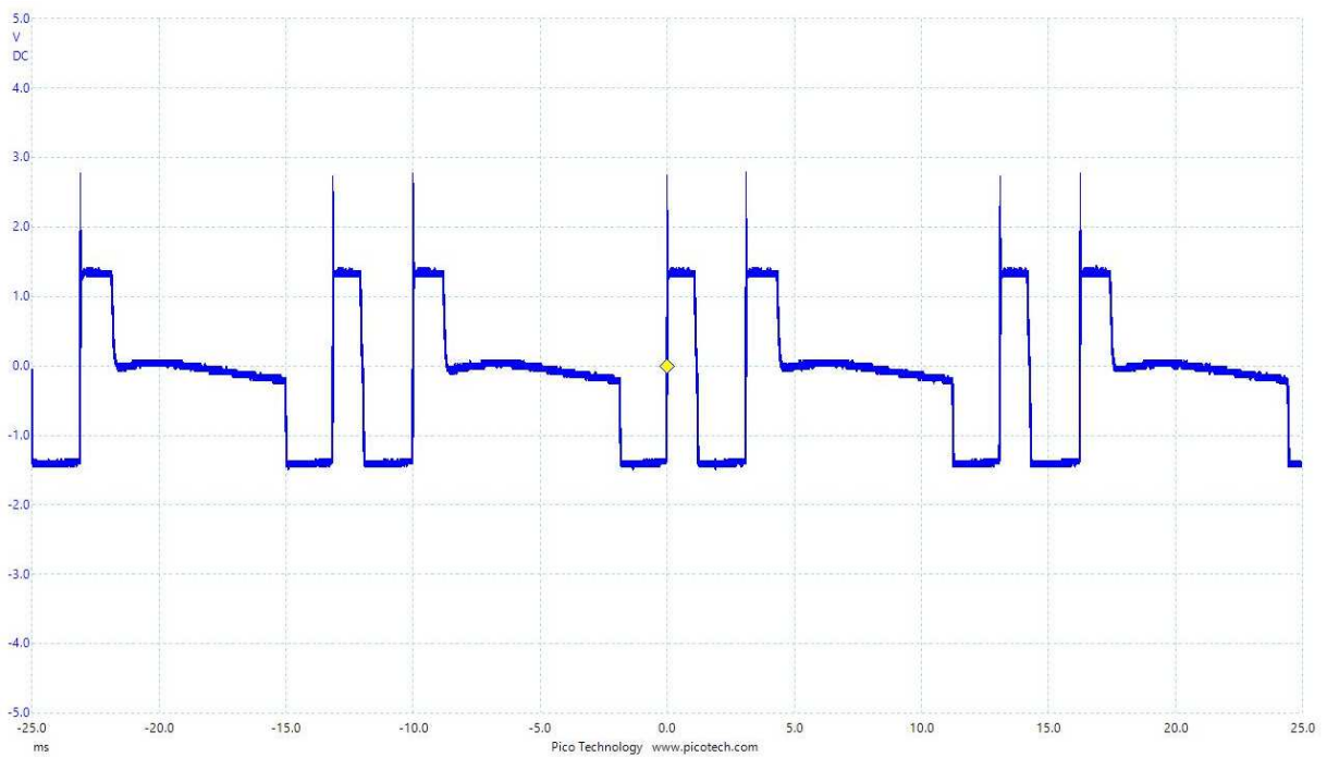
Scope measurement over 1 coil after retuning with battery @ input (probe at 10x, different scale on x-axis as screenshot above)
